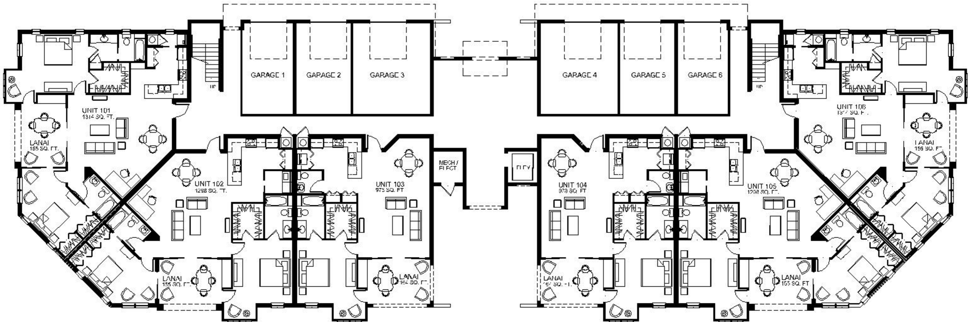
FIRST LEVEL FLOOR PLAN
